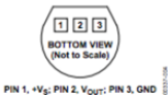
Figure 4. T-3 (TO-92)
